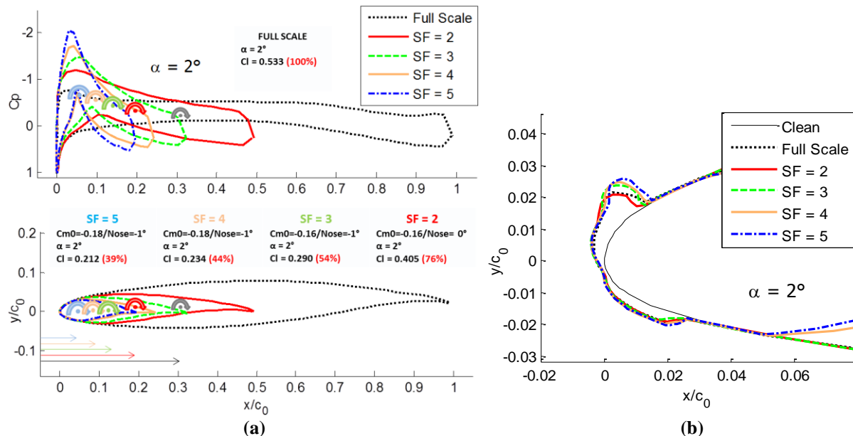
Figure 14. a) SF = 2, 3, 4, and 5 hybrid airfoils above C_p distribution at \alpha = 2^\circ b) Ice shapes
